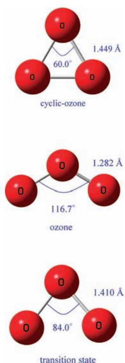
Figure 1. Calculated structures of the ozone, from top: cyclic ozone, open ozone, and the transition state.
