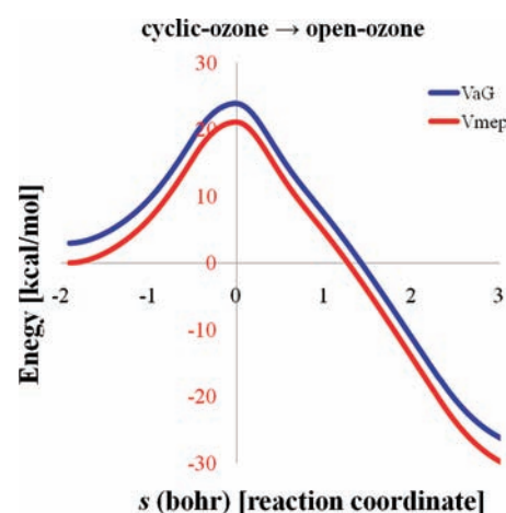
Figure 4. The calculated dual-level energy profiles along the reaction path. The V_{\text{mep}} is the relative classical (Born–Oppenheimer) energy, and the V_{\text{G}}^{\text{a}} is V_{\text{MEP}} plus the vibrational zero-point energy.
