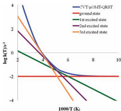
Figure 6. Arrhenius plot and the tunneling contribution from the first four reactant states to the CVT/ \mu OMT-QRST rate constants.
